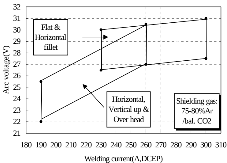
Fig.1 Recommendable welding Conditions(parameter box)
