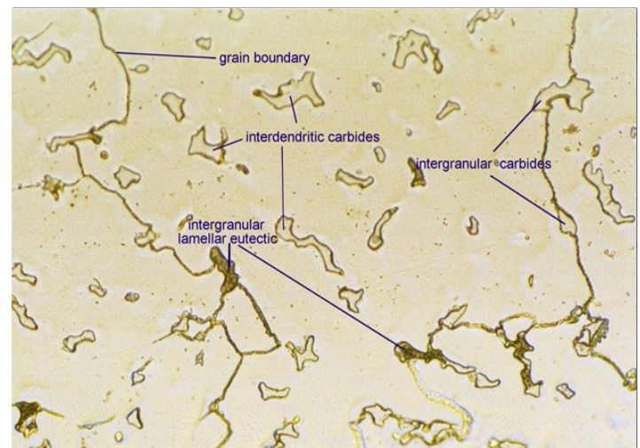
Optical Micrograph of a Stellite® 21 investment casting (as-cast, etched, 200X). The carbides in Stellite® 21 are usually of the type (Cr,Mo,Co)_{23}C_6 .
